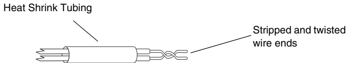
Red and Red/White Wires (VM1055CABLE)
